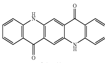
Quinacridone
