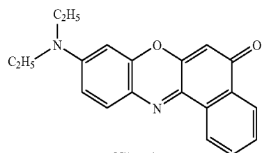
Nile red
